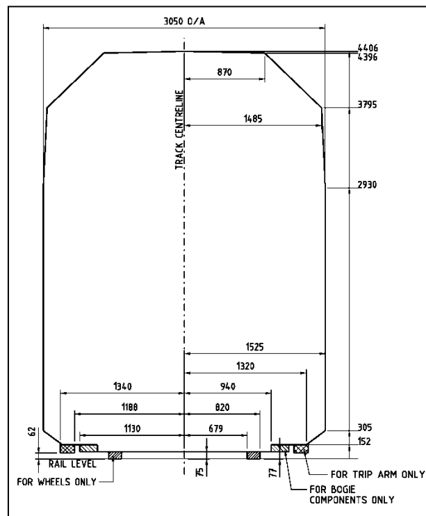
Figure A 53 - Static rolling stock outline dimensions for RISSB Reference Vehicle 27. 46
