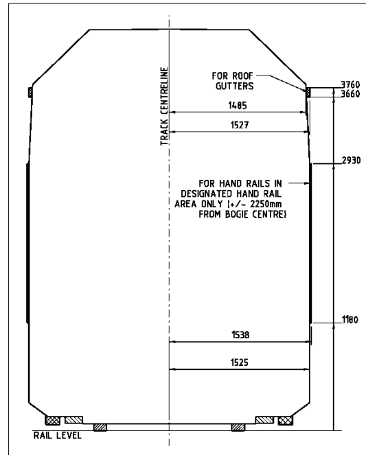
Figure B 1 - Expendable Items for RISSB Reference Vehicle 28 49
