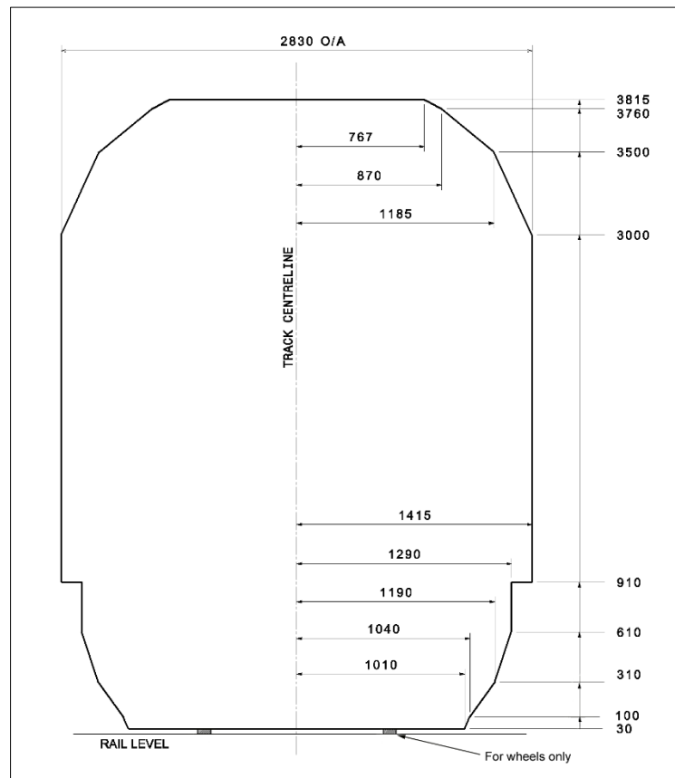
Figure A 67 - Static rolling stock outline dimensions for RISSB Reference Vehicle 34.
