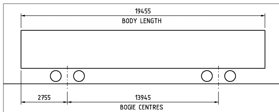
Figure A 54 - Swept outline vehicle dimensions for RISSB Reference Vehicle 27.
