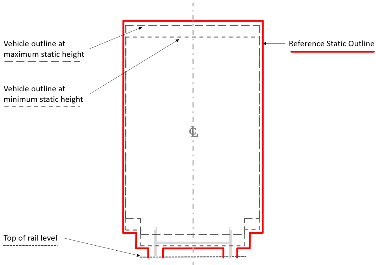
Figure 3 – Static Outline 6 .
