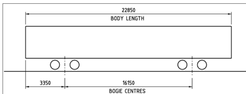
Figure A 2 - Swept outline vehicle dimensions for RISSB reference vehicle 1.
