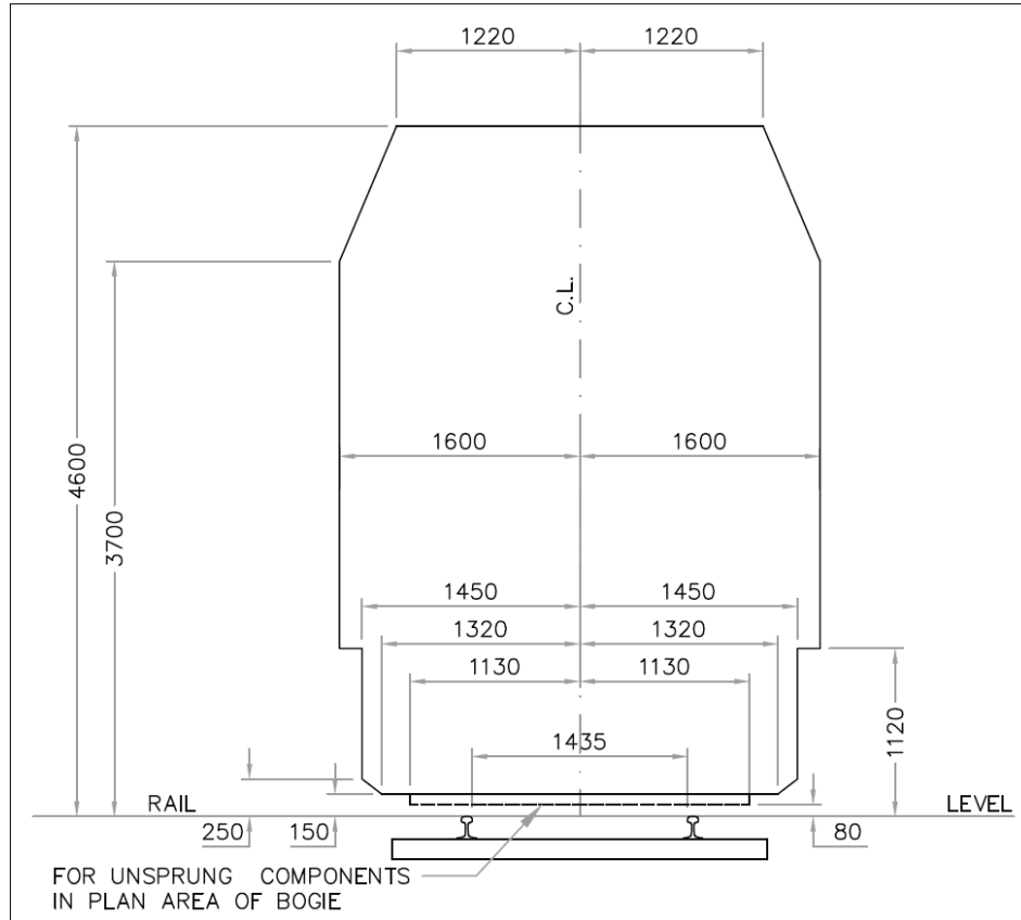
Figure A 63 - Static rolling stock outline dimensions for RISSB Reference Vehicle 32.
