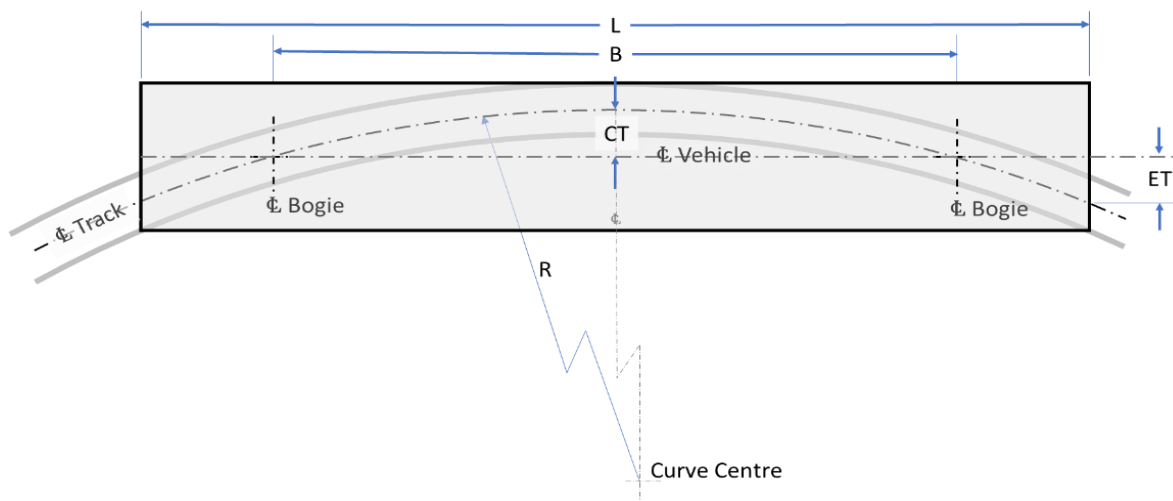
Figure 7 – Centre and End Throw 20
