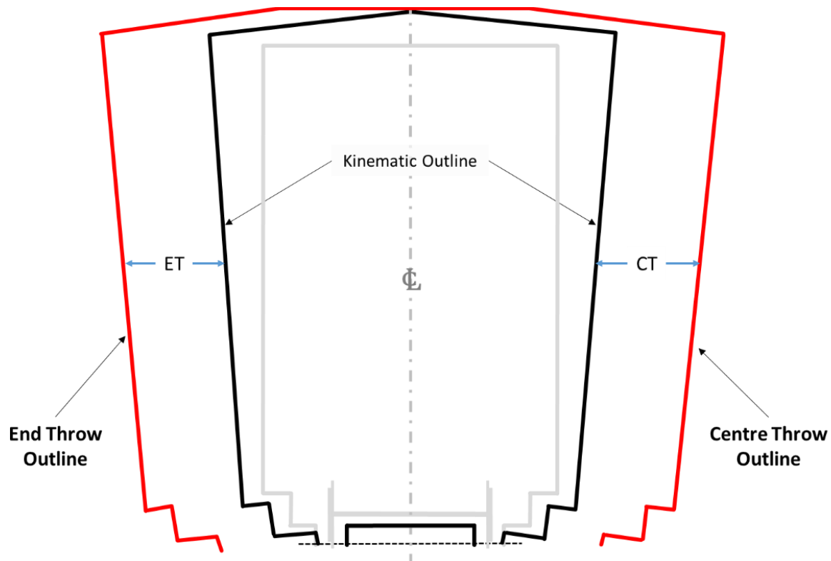
Figure 5 – Swept Outline 9
