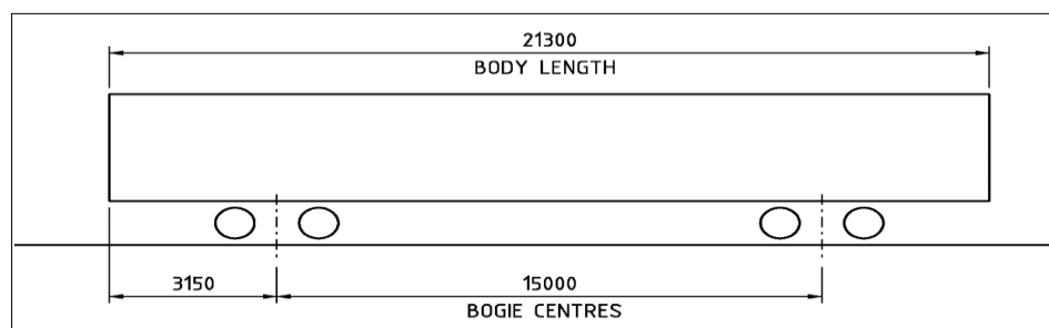
Figure A 4 - Swept outline vehicle dimensions for RISSB reference vehicle 2.
