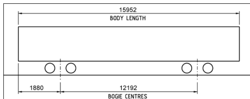
Figure A 68 - Swept outline vehicle dimensions for RISSB Reference Vehicle 34.
