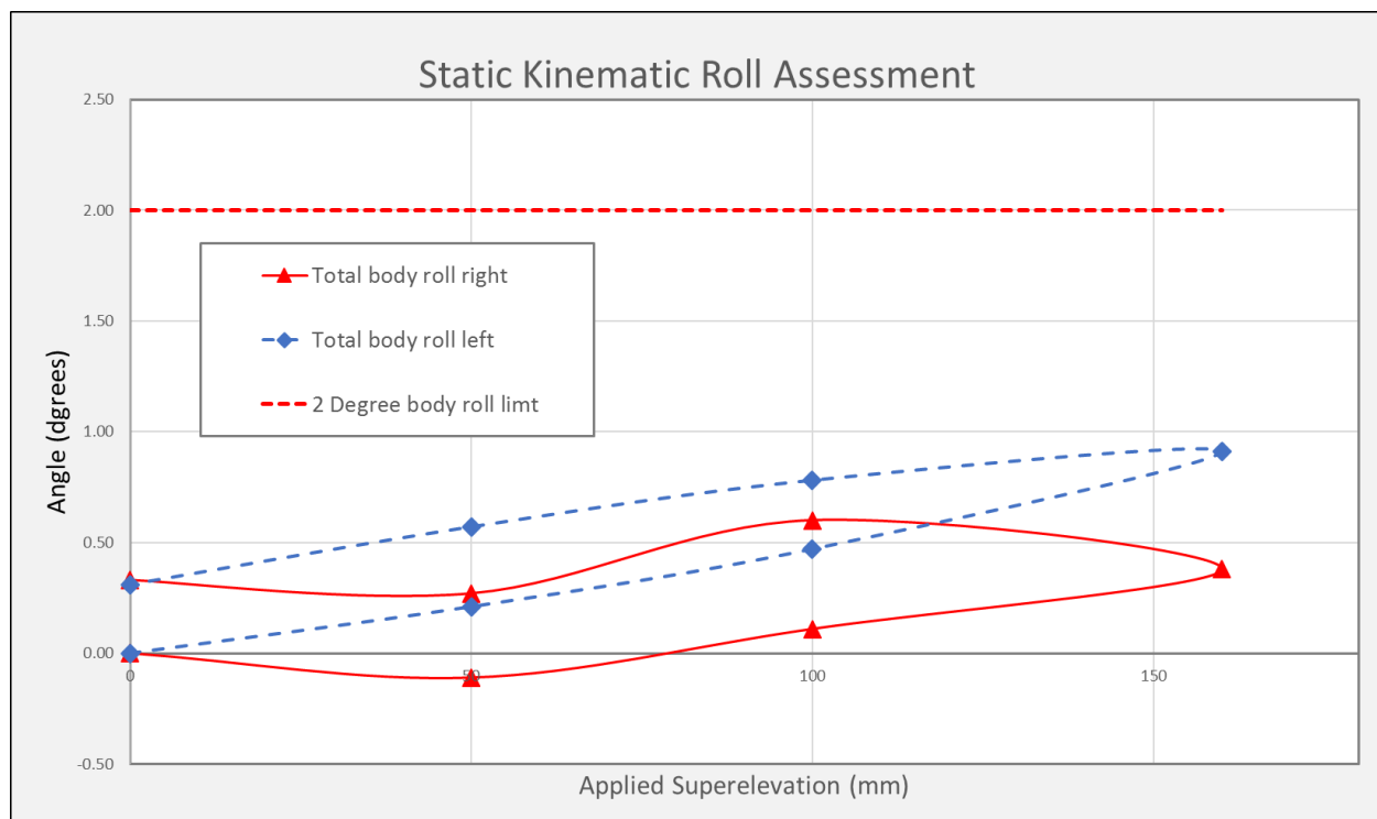
Figure C 3 - Plot of body roll vs applied superelevation
