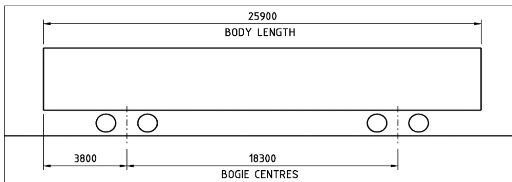
Figure A 12 - Swept outline vehicle dimensions for RISSB Reference Vehicle 6.
