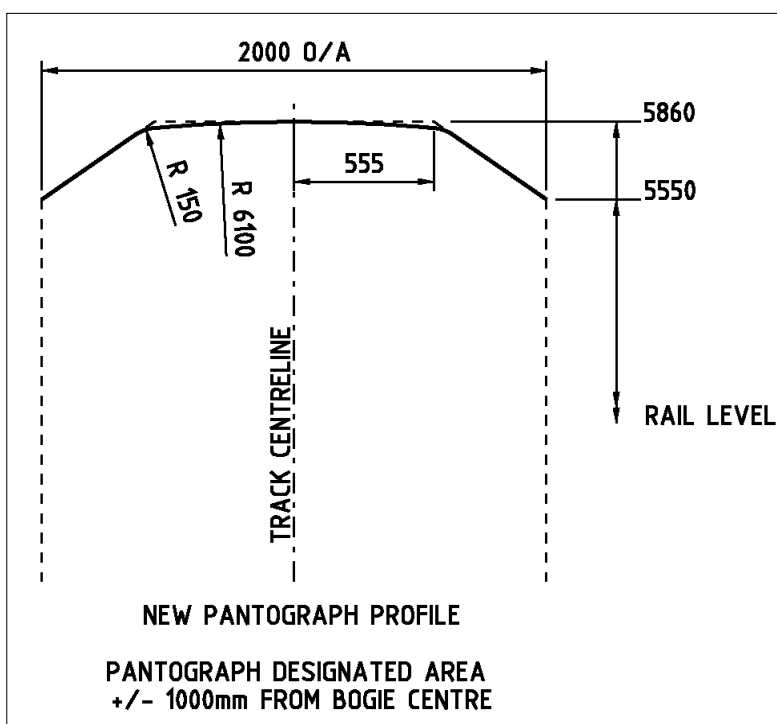
Figure B 4 - RISSB Pantograph Outline 3 52
