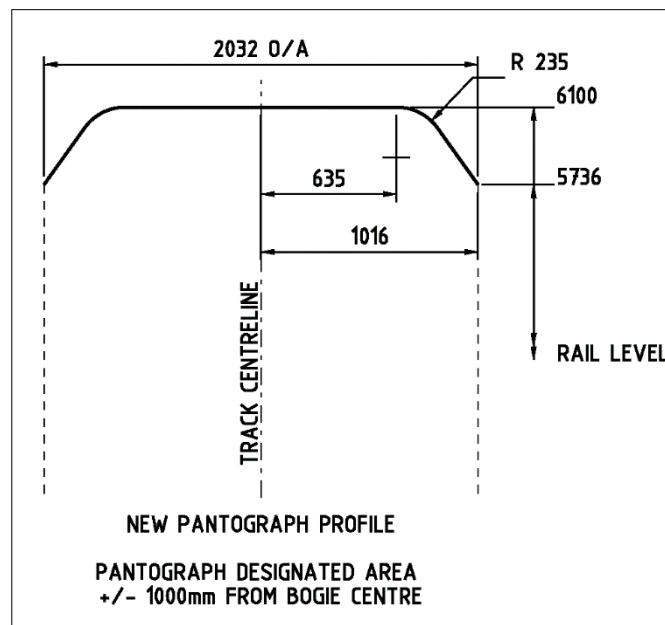
Figure B 2 - RISSB Pantograph Outline 1 50
