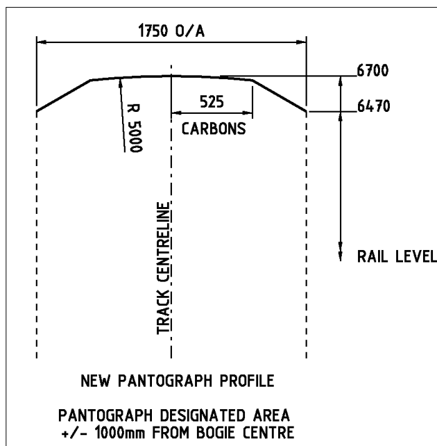
Figure B 3 - RISSB Pantograph Outline 2 51
