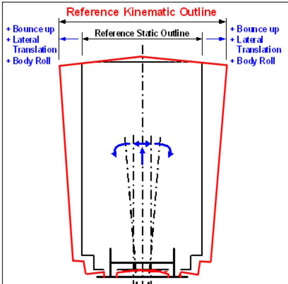
Figure 4 – Kinematic Outline 7
