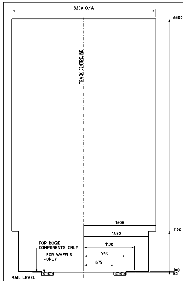
Figure A 11 - Static rolling stock outline dimensions for RISSB Reference Vehicle 6.
