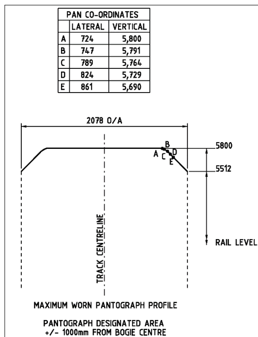
Figure B 5 - RISSB Pantograph Outline 4 53
