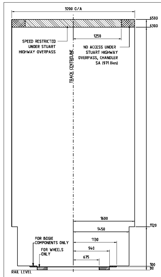
Figure A 21 - Static rolling stock outline dimensions for RISSB Reference Vehicle 11.
