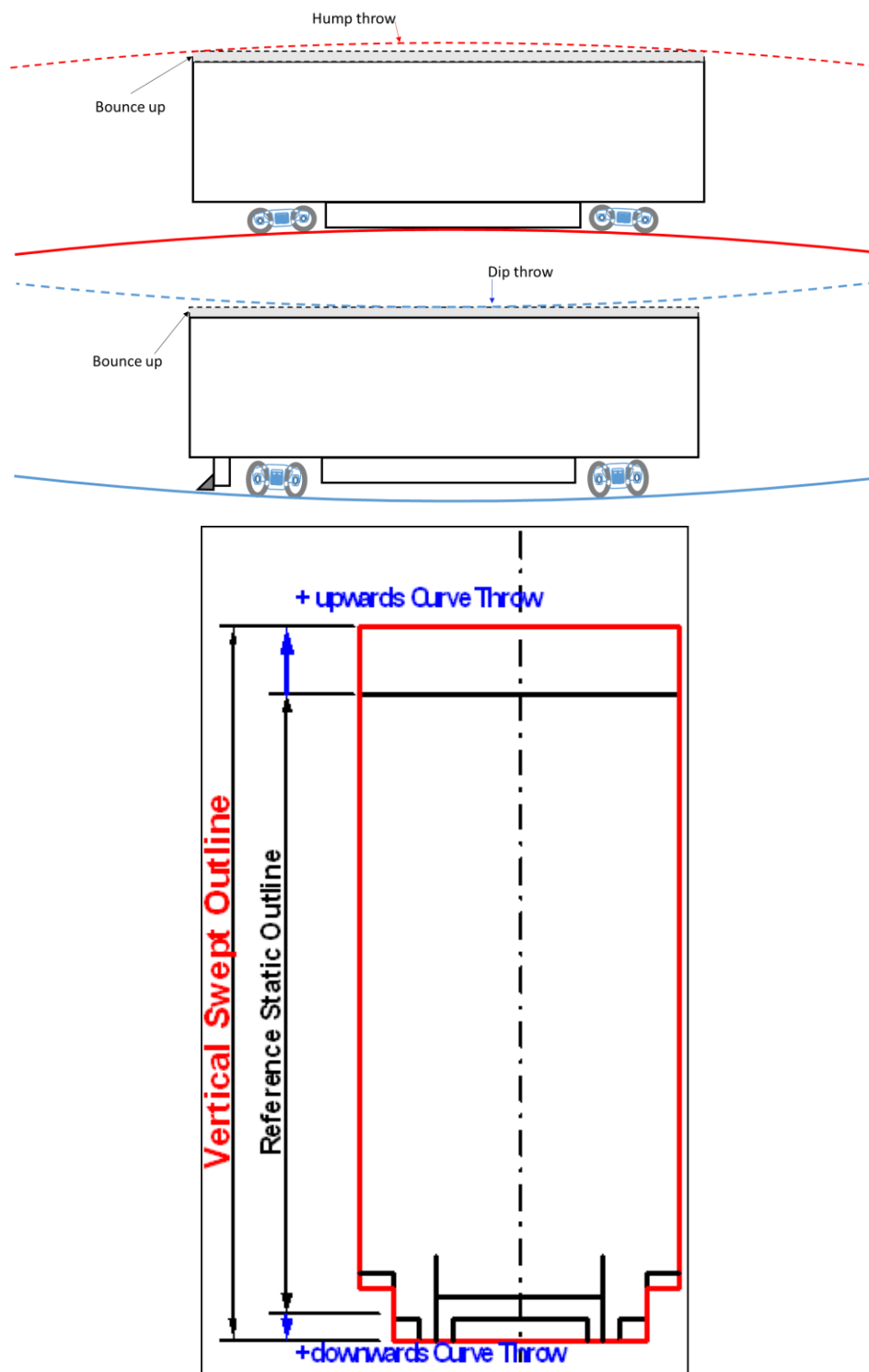
Figure 6 – Vertical Swept Outline 10
