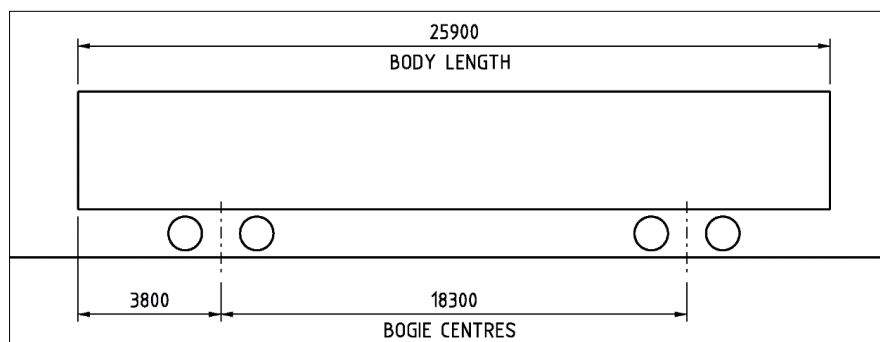
Figure A 22 - Swept outline vehicle dimensions for RISSB Reference Vehicle 11.
