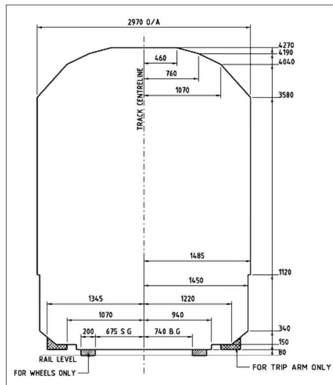
Figure A 1 - Static rolling stock outline dimensions for RISSB Reference Vehicle 1.
