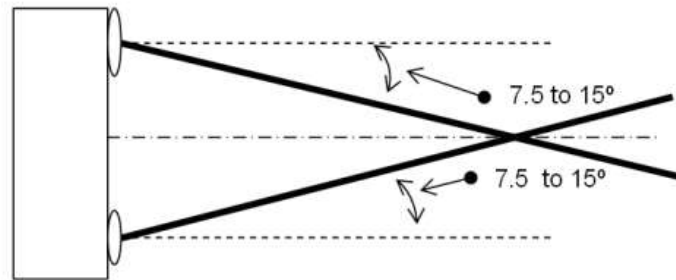
Figure 4-2 - Top View of Visibility Light Aiming (AS 7531 Figure 2)
